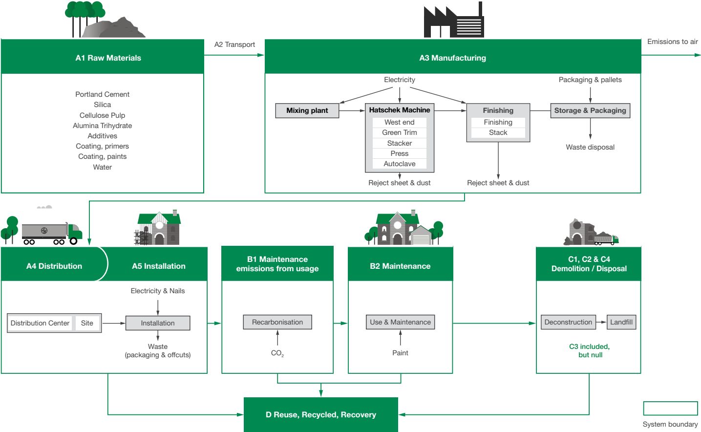
FIGURE 1. SYSTEM BOUNDARY
